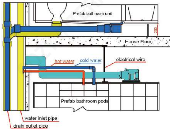
Horizontal drain style
