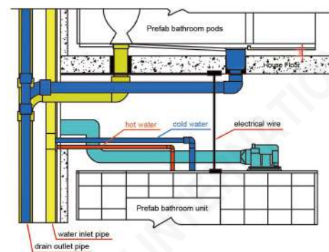
Vertical drain style
