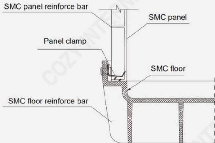
Diagram for panels and floor
